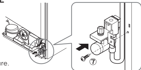
housing refrigerator bottom
