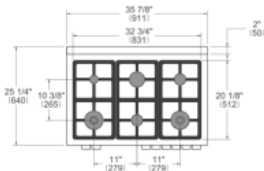
WORKTOP DETAILS
