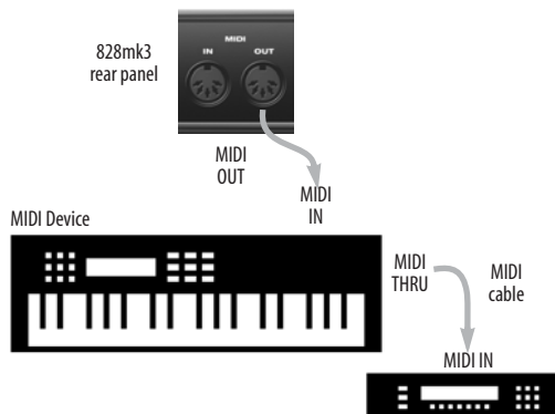
Figure 4-10: Connecting additional devices with MIDI THRU ports.
