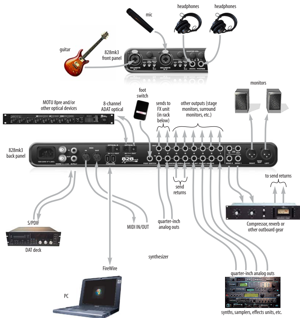
Figure 4-11: A typical 828mk3 studio setup.
