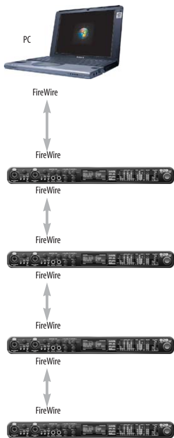
Figure 4-21: Connecting multiple 828mk3 interfaces (or other MOTU FireWire audio interfaces) to a computer.
