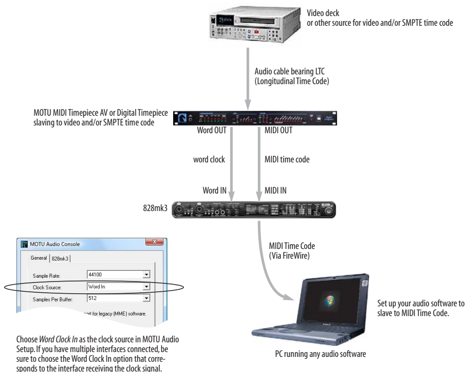
Figure 4-17: If your host audio software does not support sample-accurate sync and the 828mk3's built-in SMPTE sync features, use a universal synchronizer such as the MOTU MIDI Timepiece AV or Digital Timepiece.
