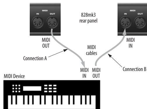
Figure 4-9: Connecting a MIDI device to the 828mk3.
