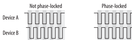
Figure 4-14: When transferring audio, two devices must have phase-locked audio clocks to prevent clicks, pops or other artifacts.
