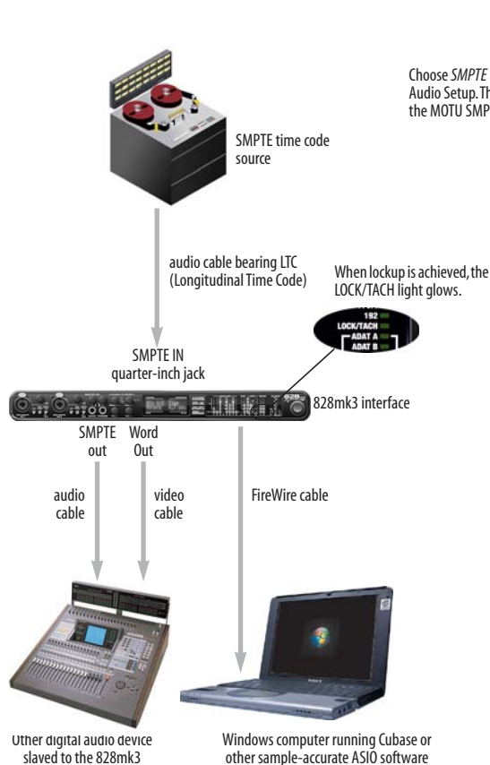
Figure 4-16: Connections for synchronizing the 828mk3 directly to SMPTE time code.
