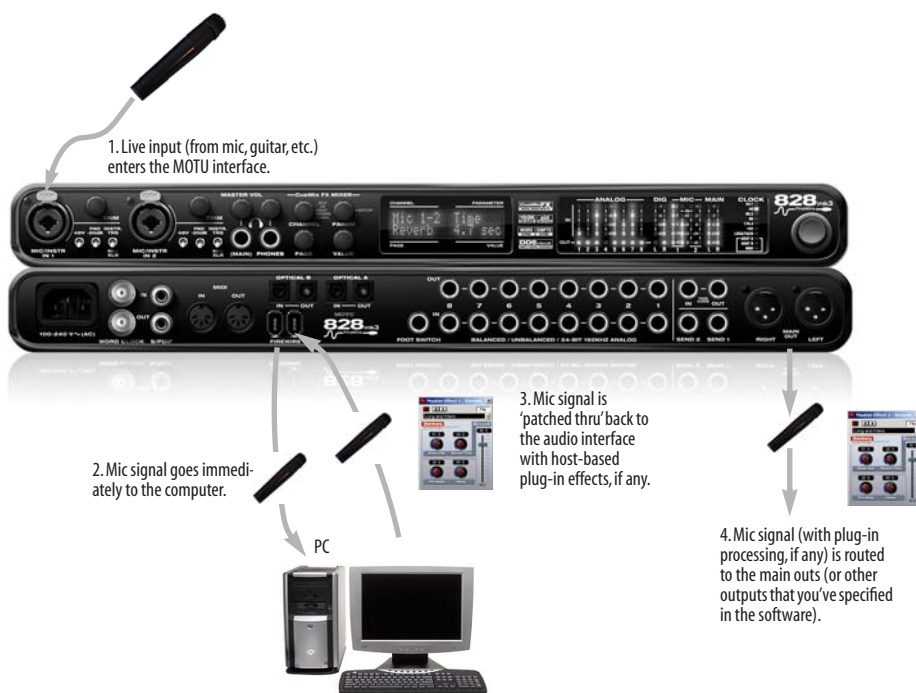
Figure 10-1: There are two ways to monitor live audio inputs with an 828mk3: 1) through the computer or 2) via CueMix FX hardware monitoring. This diagram shows method 1 (through the computer). When using this method, use your host software's buffer setting to reduce the slight delay you hear when monitoring the live input, but don't lower it too much, or your computer might get sluggish.
