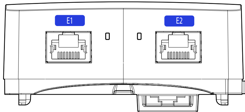
Figure 3 AP-503H (bottom view)
