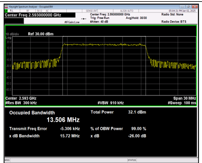
Band41-15MHz-16QAM-39725-75RB#0
