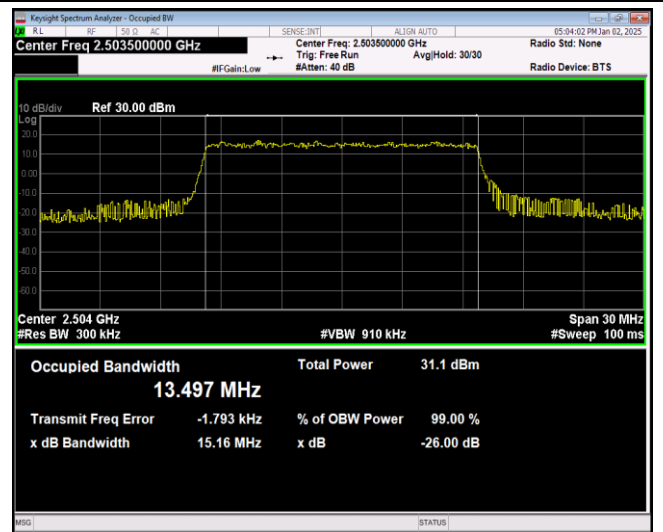
Band41-15MHz-16QAM-41515-75RB#0
