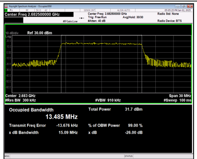
Band41-15MHz-64QAM-40620-75RB#0
