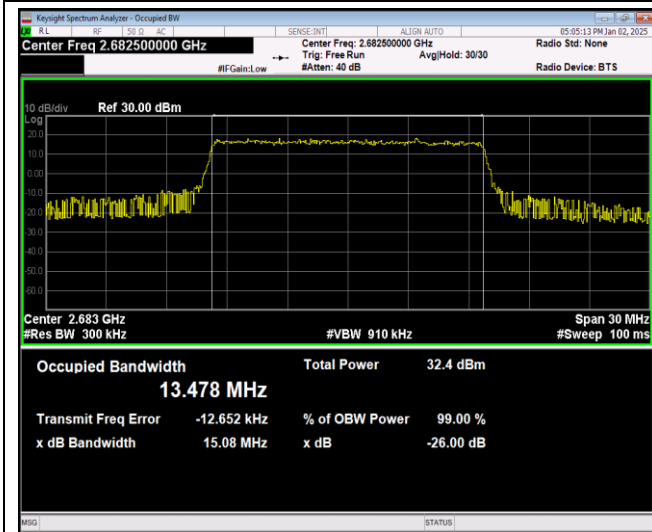
Band41-15MHz-16QAM-40620-75RB#0
