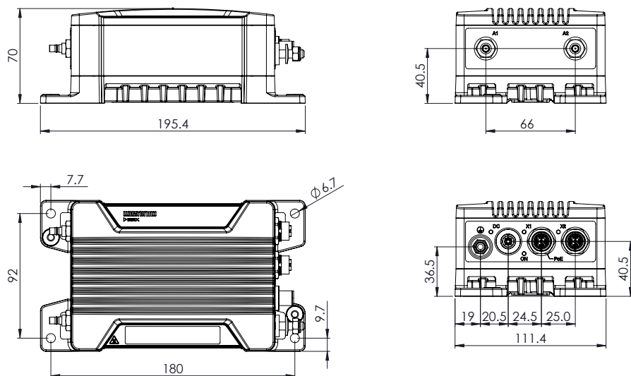
Figure 5. Dimensional drawing
