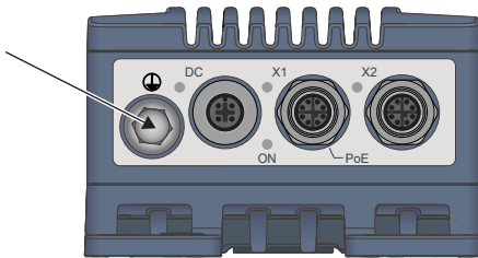
Figure 6. Earth connection
