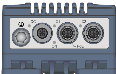
Figure 4. LED indicators
