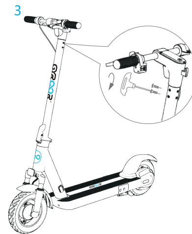
3. Use the hexagon wrench in the box to tighten the screws on both sides and the back of the handlebars.
