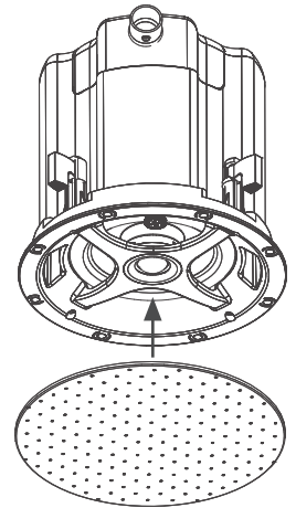
FIGURE 15: GRILLE INSTALLATION
