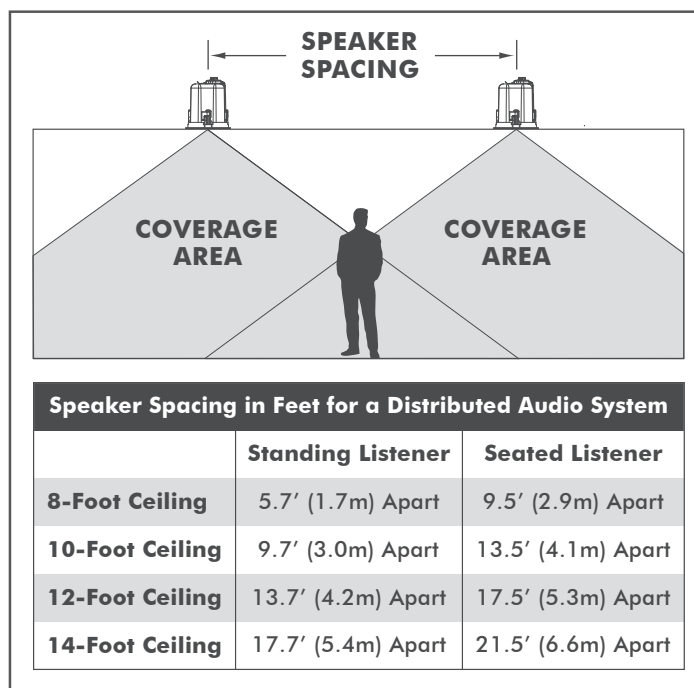
FIGURE 2: SPEAKER SPACING
