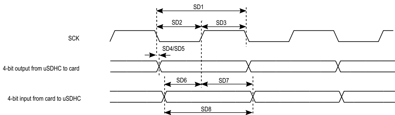
Figure 41. SDR50/SDR104 timing
