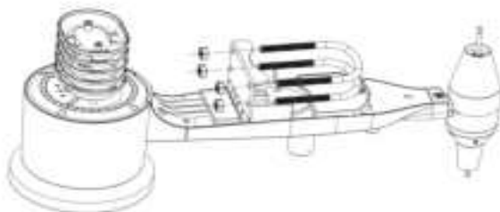
Figure 1: U-bolt Installation
