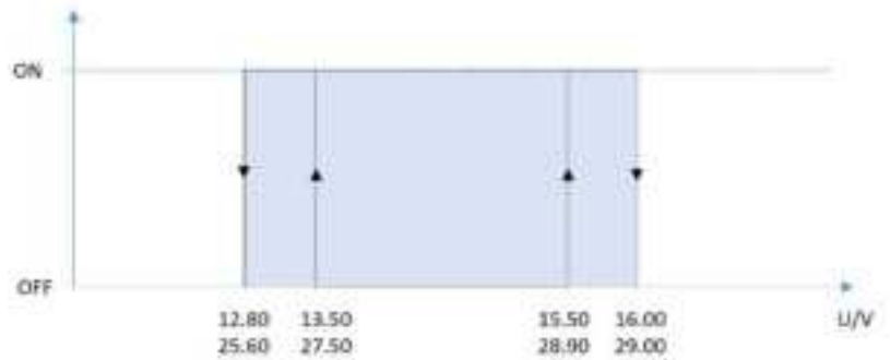
Fig. 3: Switch-on / off voltage CDR 12/24 V
