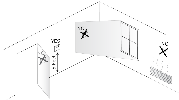
Figure 52. Thermostat/sensor location
