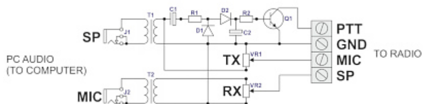
Example connection using the DIGIVOX-2 modem
