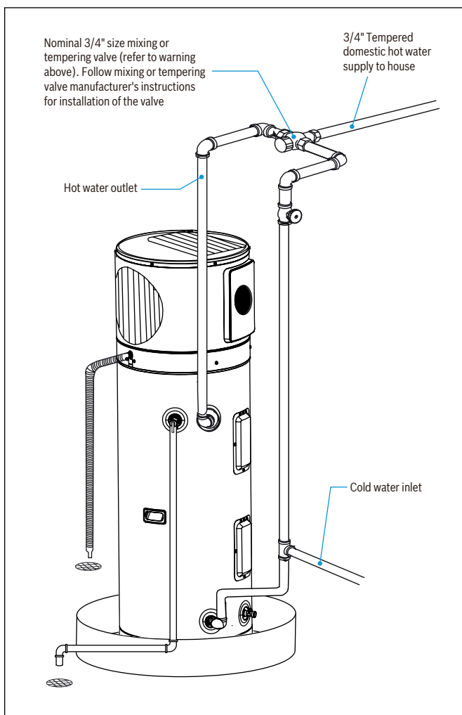
Figure 13 Installation with thermostatic mixing valve
