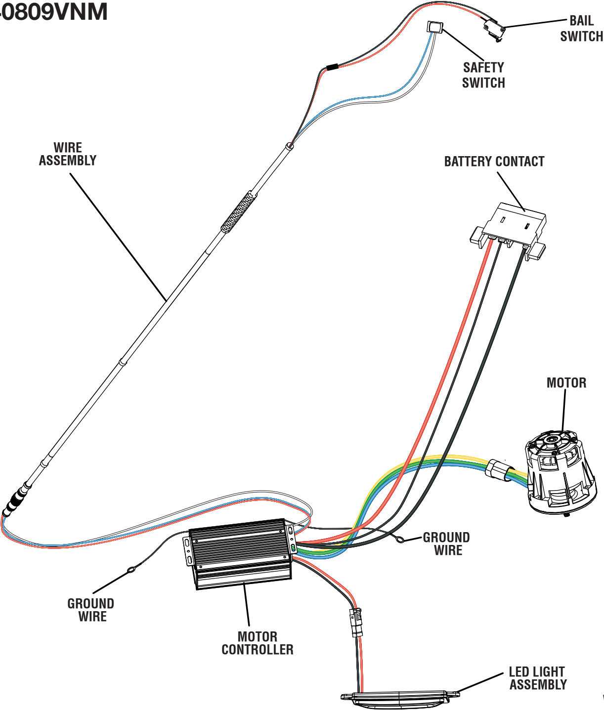
WIRING DIAGRAM
