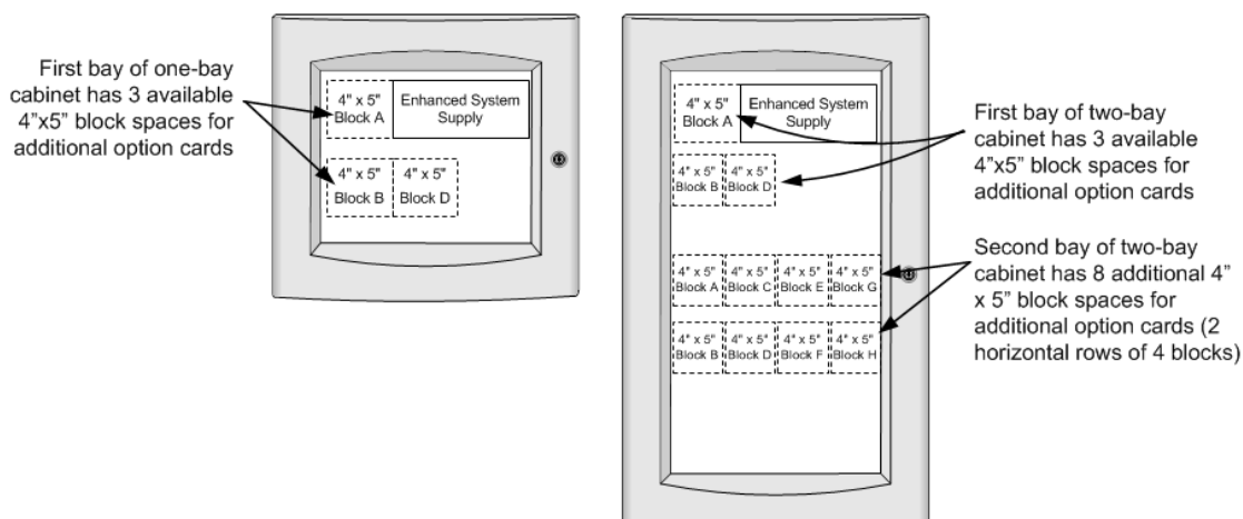
Figure 17: Cabinet one and two bay loading reference
