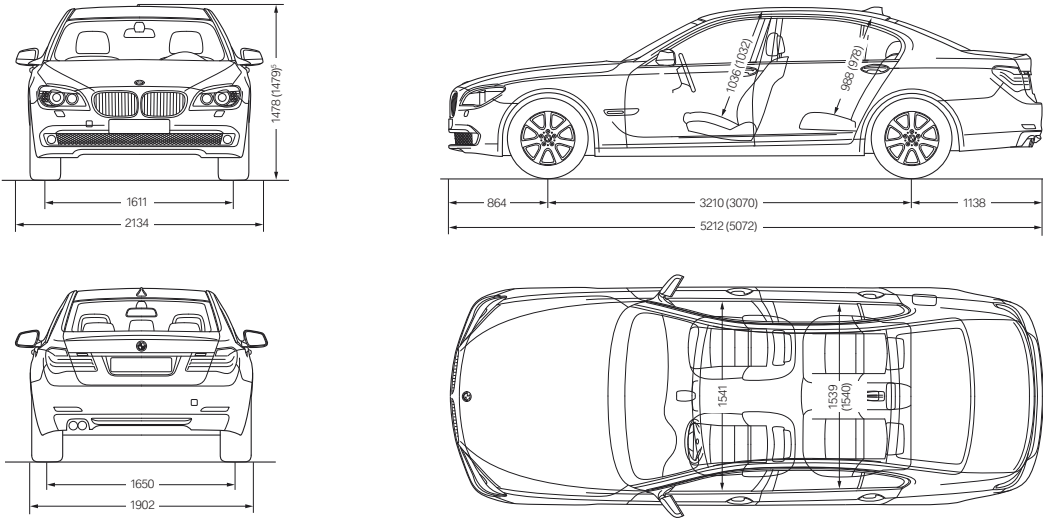
All dimensions in the technical drawings are given in millimetres. Luggage compartment volume 500 litres. Figures in ( ) refer to 7 Series short-wheelbase version.
