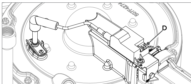
Fig. 9 - Igniter Kit Installed
