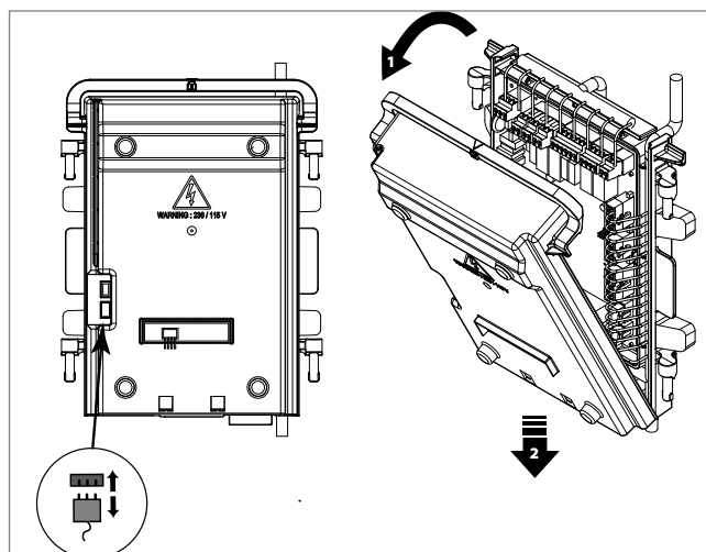
Fig. 11 - Removal of Control Box Front Cover
