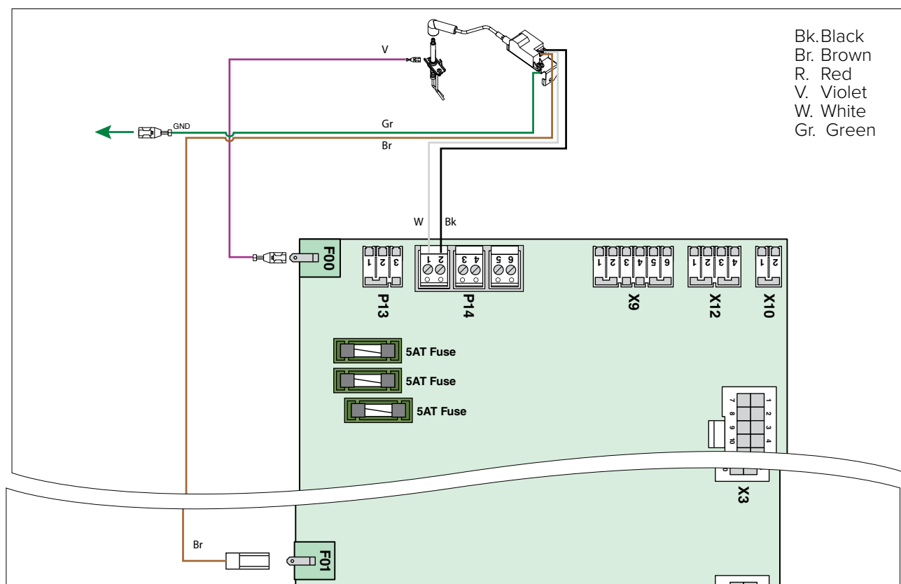
Fig. 18 - Control Module Wiring - Post-modification
