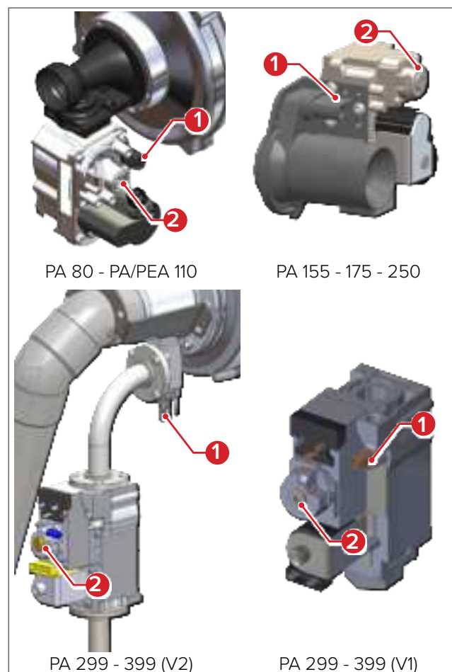
Fig. 20 - Position of Throttle and Offset Screws
