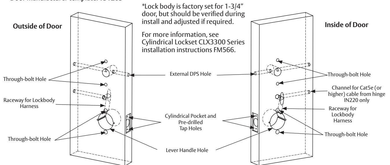
Figure 5-1B Wood Door Preparation
