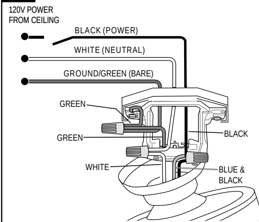
FAN CONTROLLED BY PULL CHAIN, LIGHT BY WALL SWITCH
