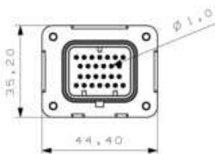
Figure 3 Schematic diagram of connector appearance
