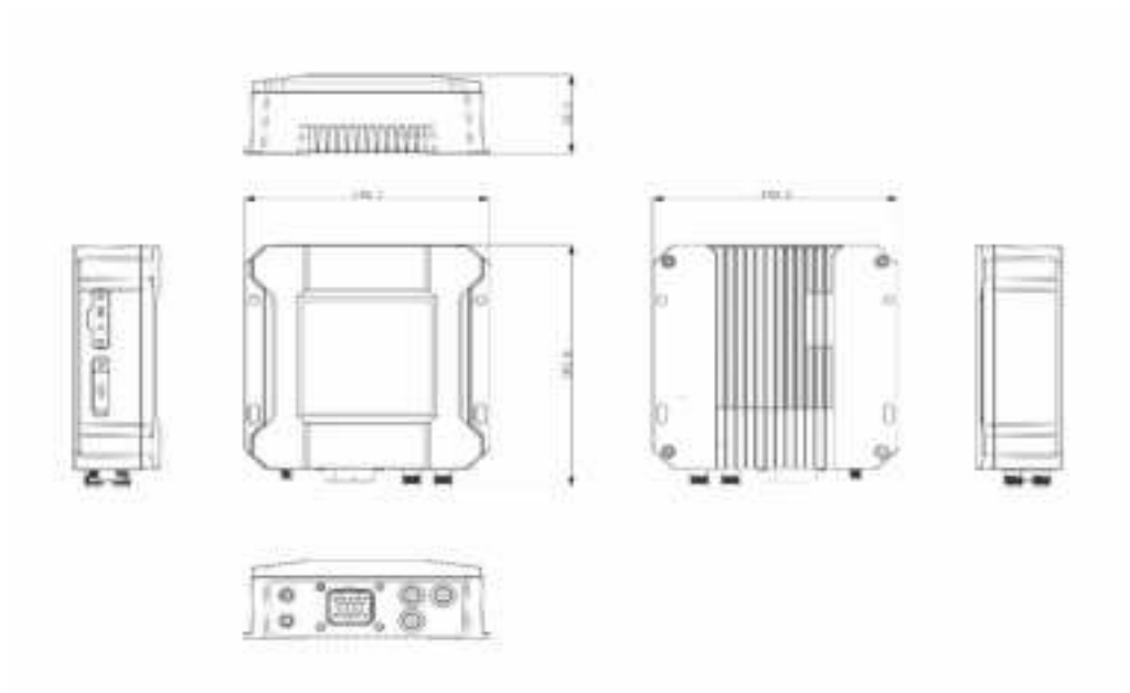
Figure 2 R62 Dimensions
