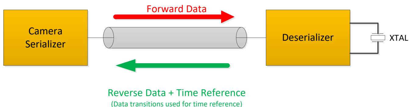
Figure 20: RoR Operation
