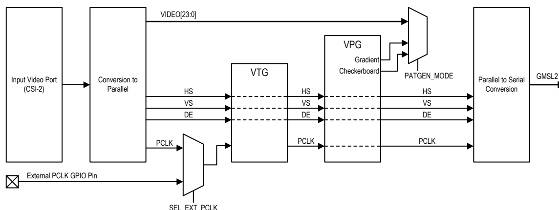
Figure 38. Video Path Through VTG and VPG
