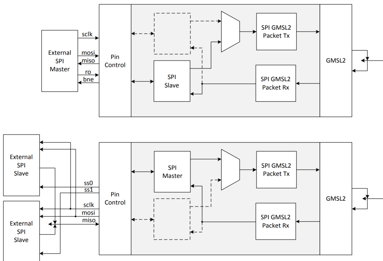
Figure 10. SPI Architecture
