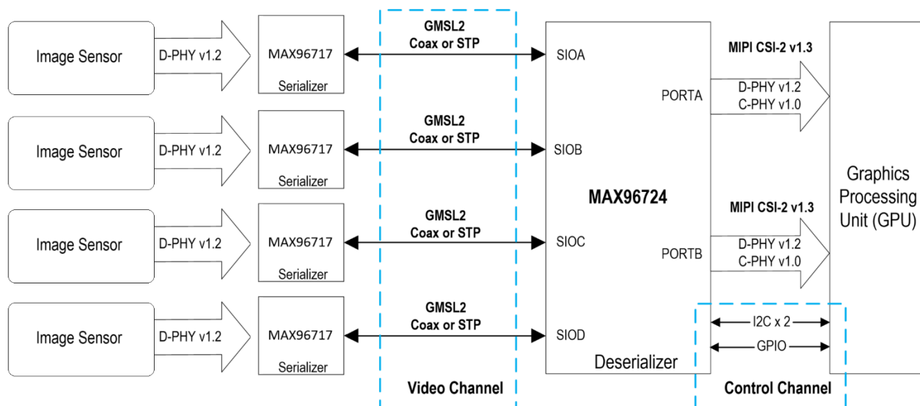
Figure 1. MAX96717 Four-Camera Application Example
