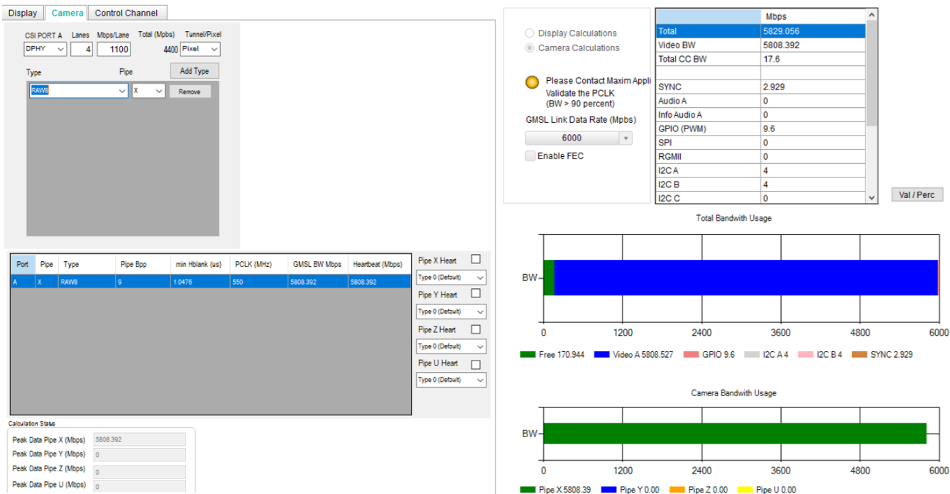
Figure 31. Bandwidth Calculations without Doubling
