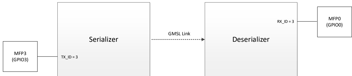
Figure 34. GPIO Forwarding Example with a Transition from MFP3 to MFP0
