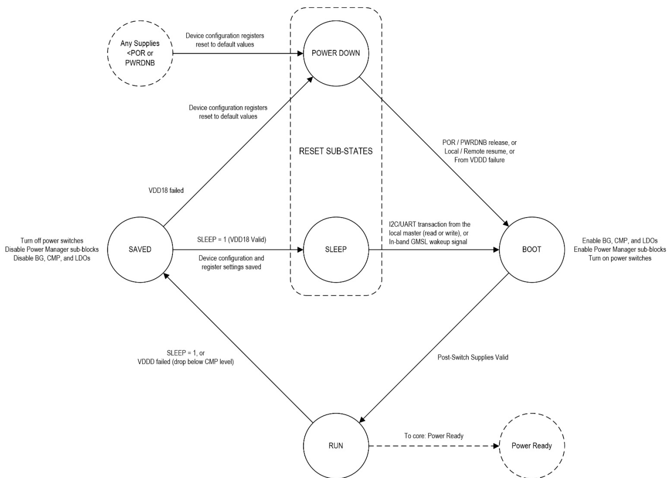
Figure 19. Power Manager State Diagram
