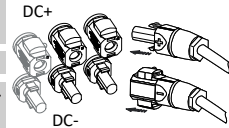
Fig. 11: Connection to XL version
