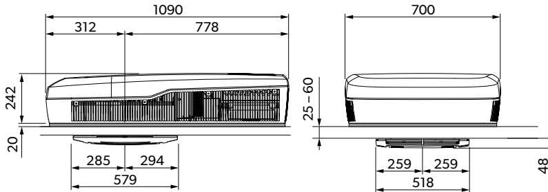
FreshJet FJX7337IHP
