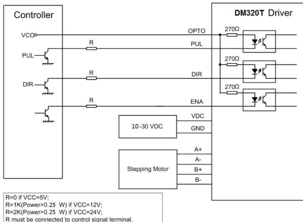
Figure 9: Typical connection
