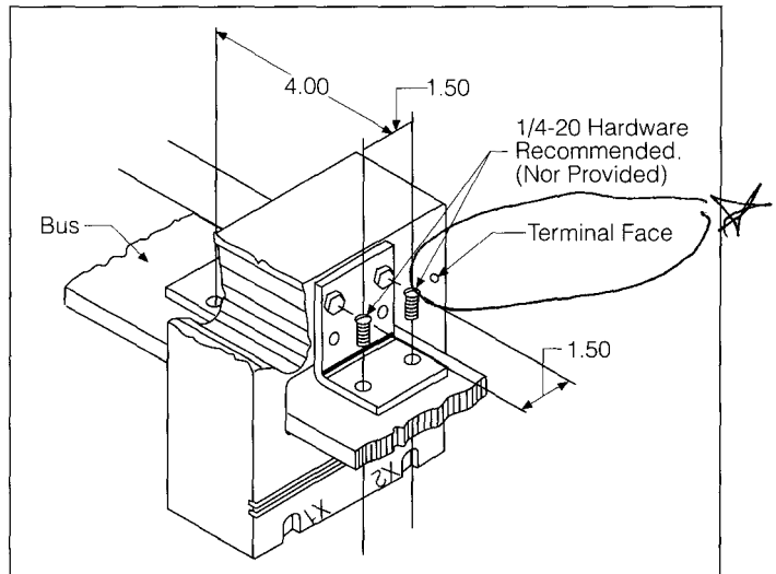
Bus Mounting
