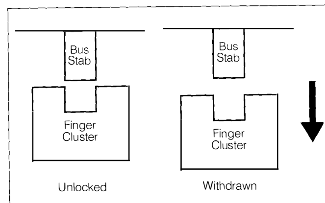
Withdrawn Position
