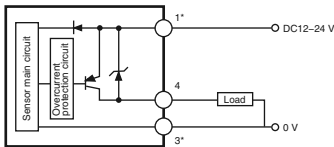
Output Circuit Diagram
