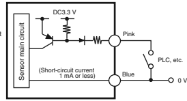
Input Circuit Diagram (FS-N13N/N14N only)
