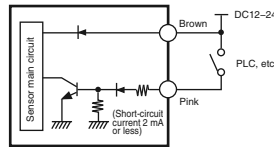
Input Circuit Diagram (FS-N13P/N14P only)
