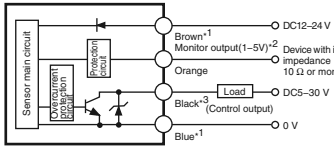
Output Circuit Diagram
