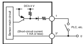
Input Circuit Diagram
