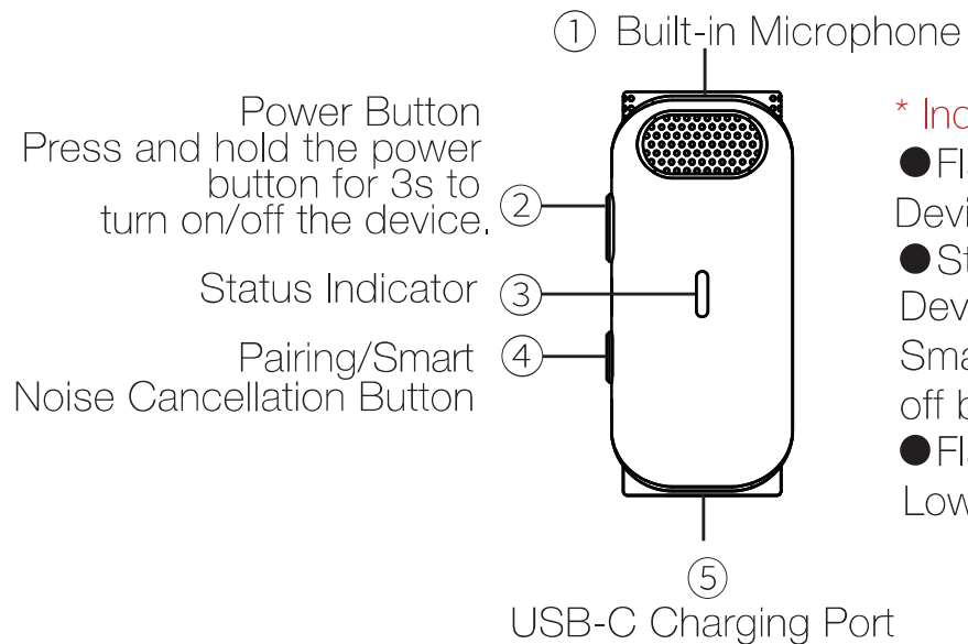
TX: Transmitter
