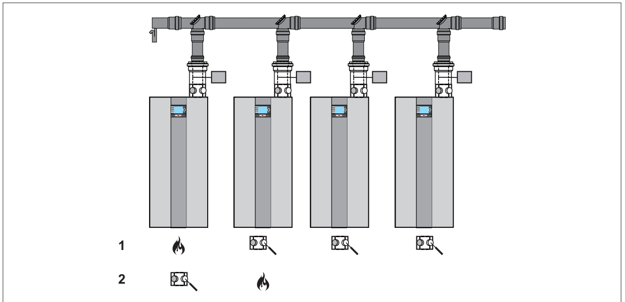
Afb. 6.7 Rookgascascade
