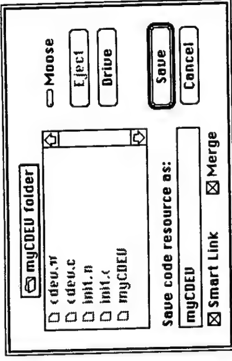
Figure 7-10 The Merge check box in the Build Code Resource... dialog
