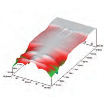
Directivity of a single speaker
