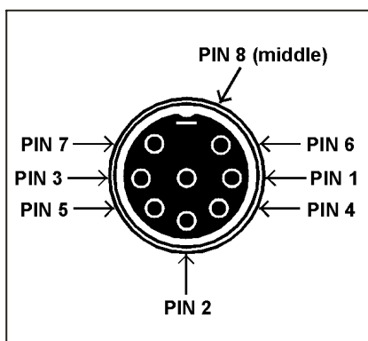
Figure 6 - 5: Remote Switches
