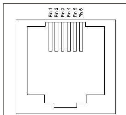
Figure 6 - 7: RJ12 Connector
