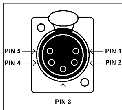
Figure 6 - 6: DMX Connector
