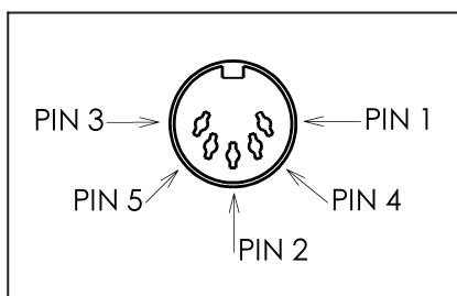
Figure 6 - 4: MIDI Connector
