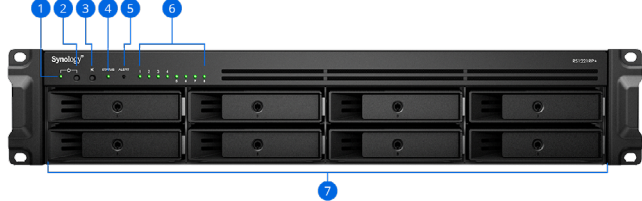
Front (RS1221RP+)
