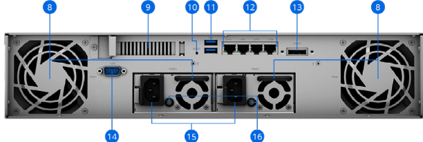
Rear (RS1221RP+)
