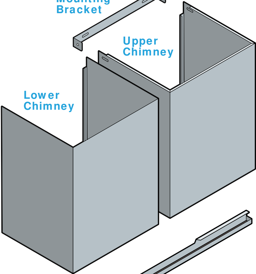
Grease Tunnel
