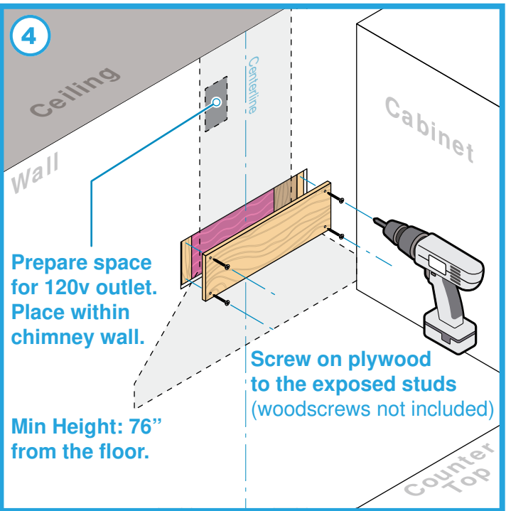
(4) Screw on plywood to the exposed studs (woodscrews not included). Prepare space for 120v outlet. Place within chimney wall, hidden from view. Min Height: 76" from the floor.
