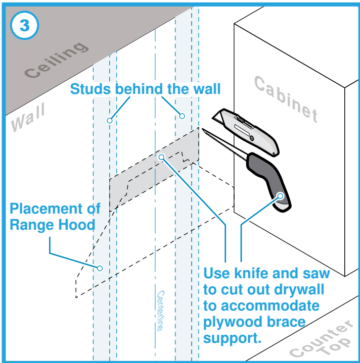
(3) Use knife and saw to cut out drywall to accommodate a plywood brace support. The inserted plywood should be the same depth as the drywall slab it is replacing.
