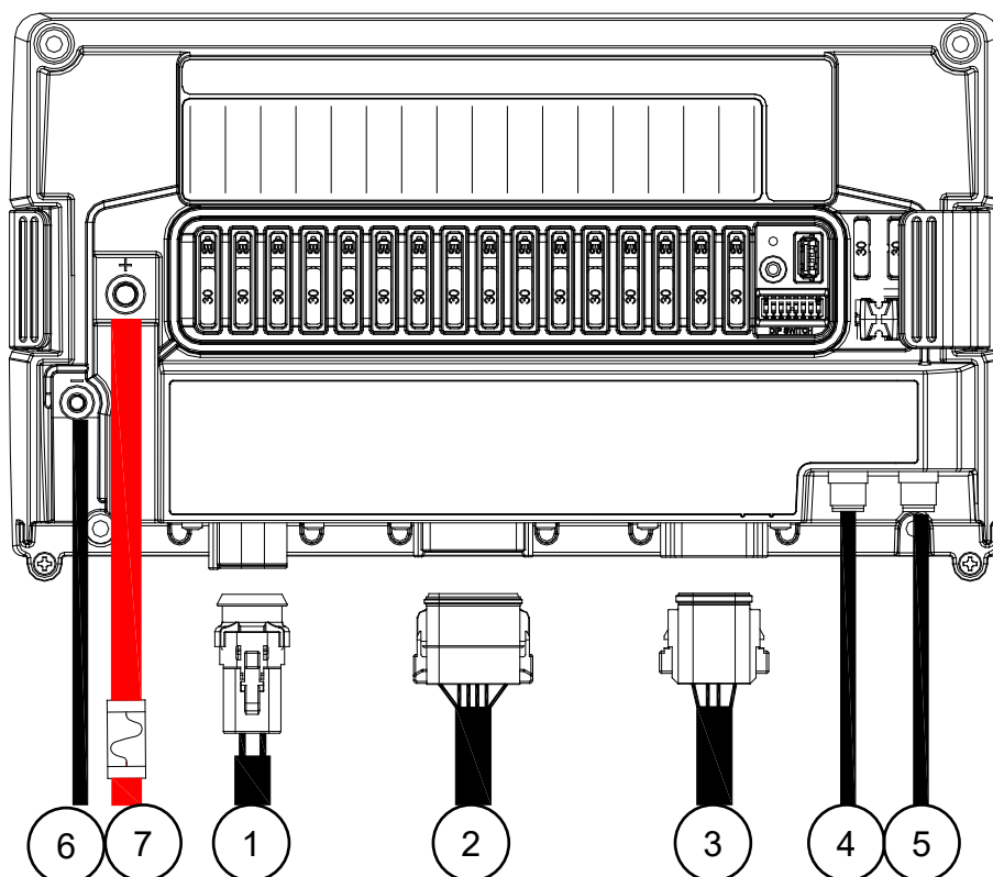
Figure 10. Control 1 Connections
