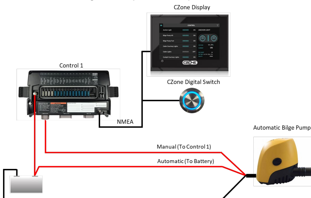
Figure 7. Control 1 Bilge Pump Wiring Example
