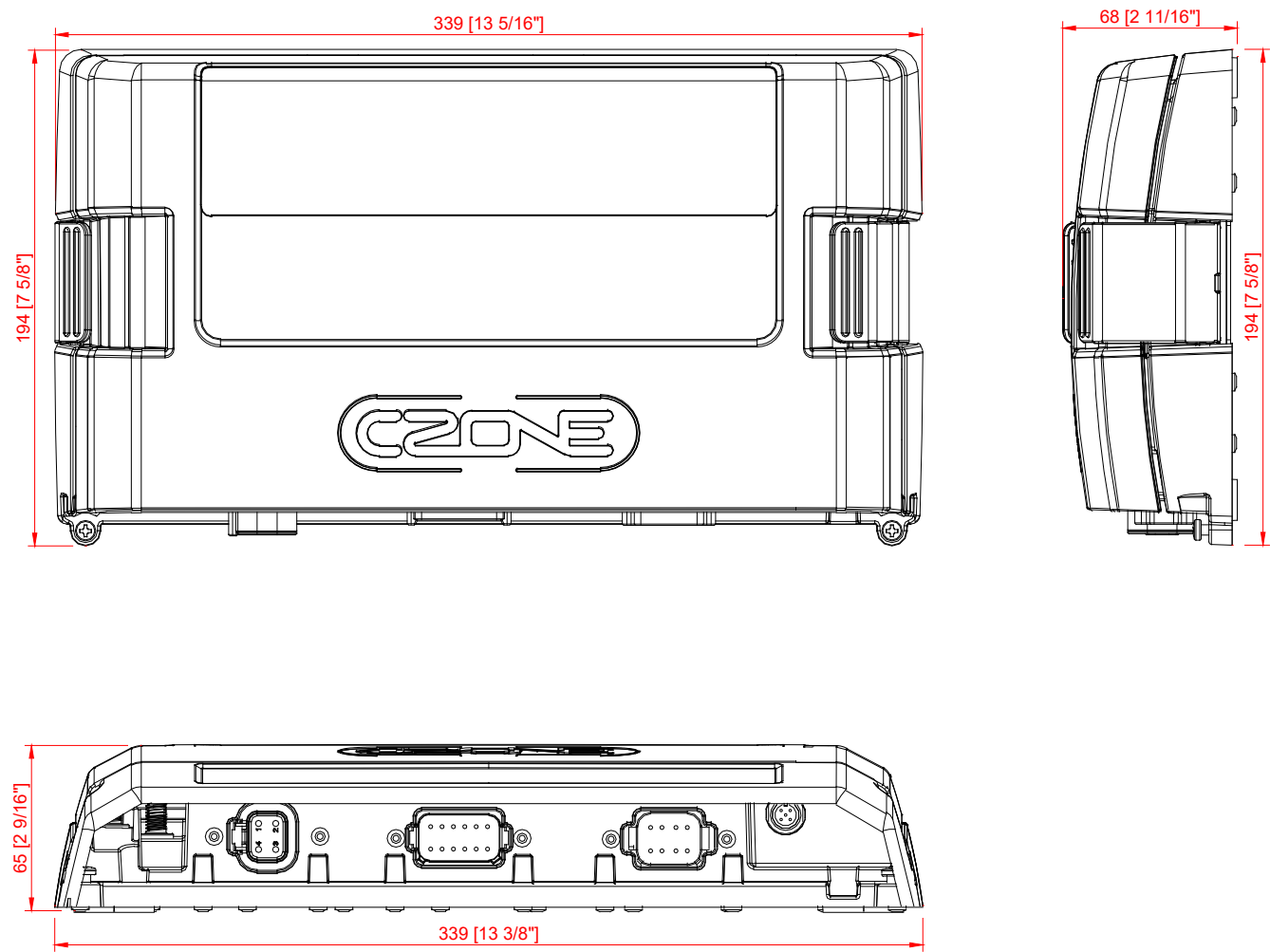
Figure 13. Control 1 Dimensions
