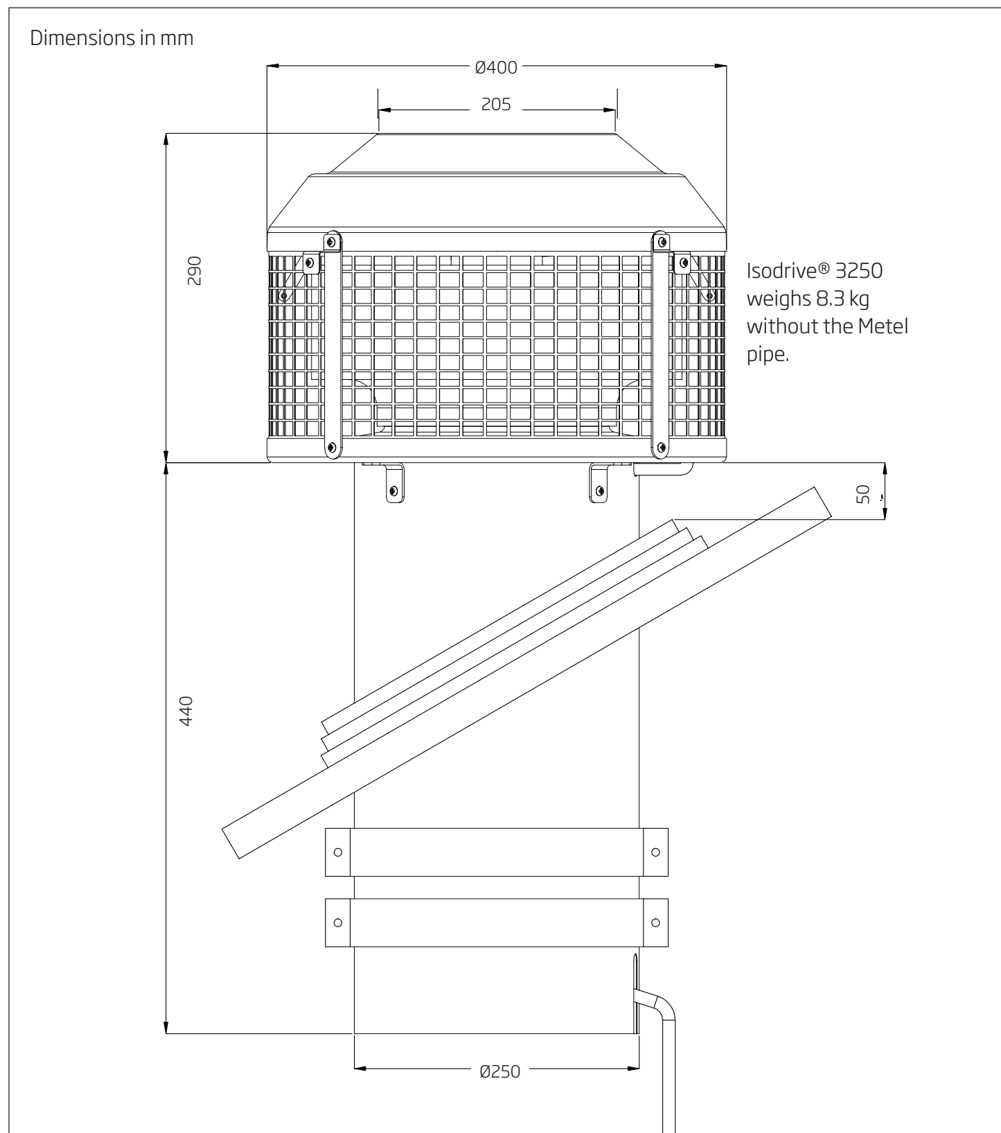
Figure 7: Measurements for Isodrive 3250
