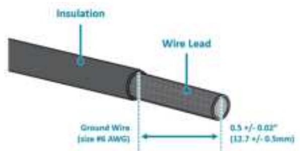
6-AWG wire for grounding
