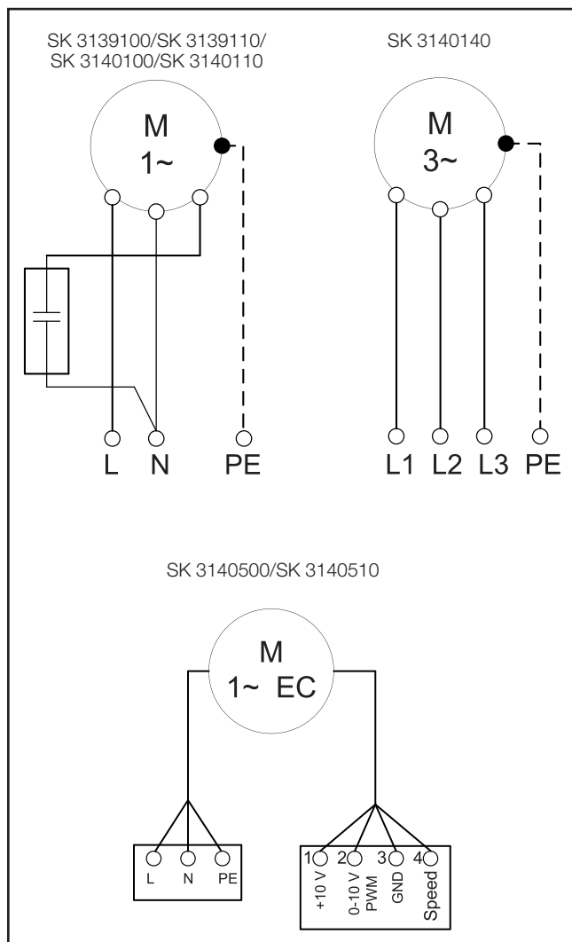
Fig. 2: Connection diagrams
