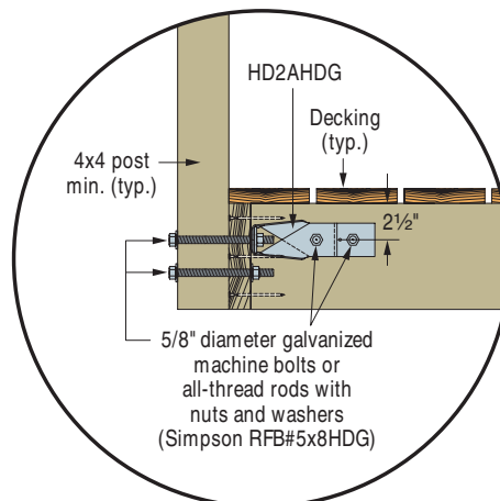
HD2A installed as a lateral anchor for a deck guardrail post. Refer to technical bulletin T-HD2AGRDL for more information. (See page 187 for details)
