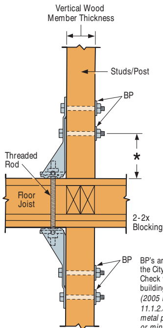
Typical HD5A Tie Between Floors
