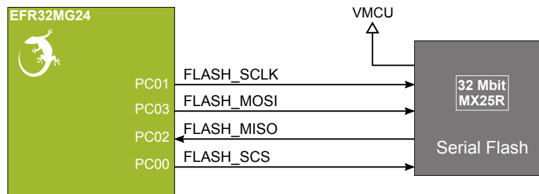
Figure 3.6. Serial Flash
