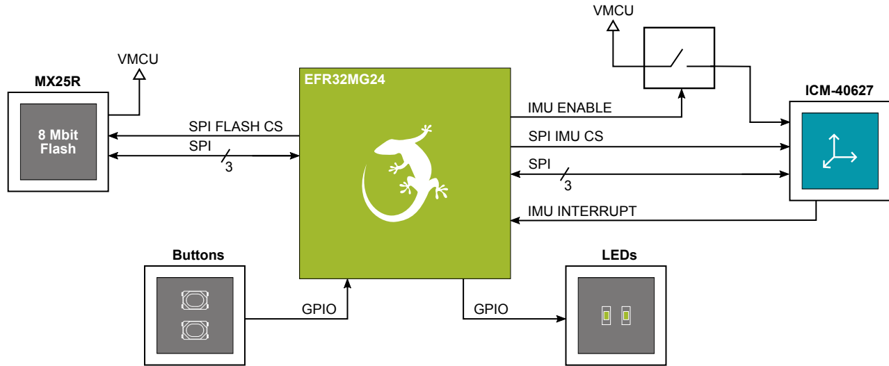
Figure 3.3. Peripherals
