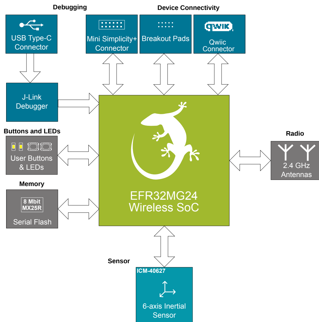
Figure 3.1. EFR32xG24 Channel Sounding Dev Kit Block Diagram
