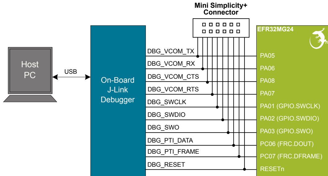
Figure 3.8. On-Board Debugger Connections
