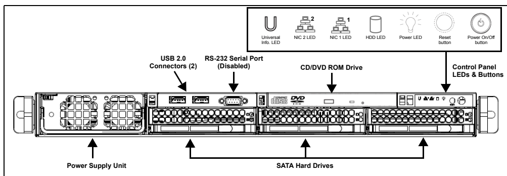
Figure 1-1. Front panel components of the Intuition XG-e
