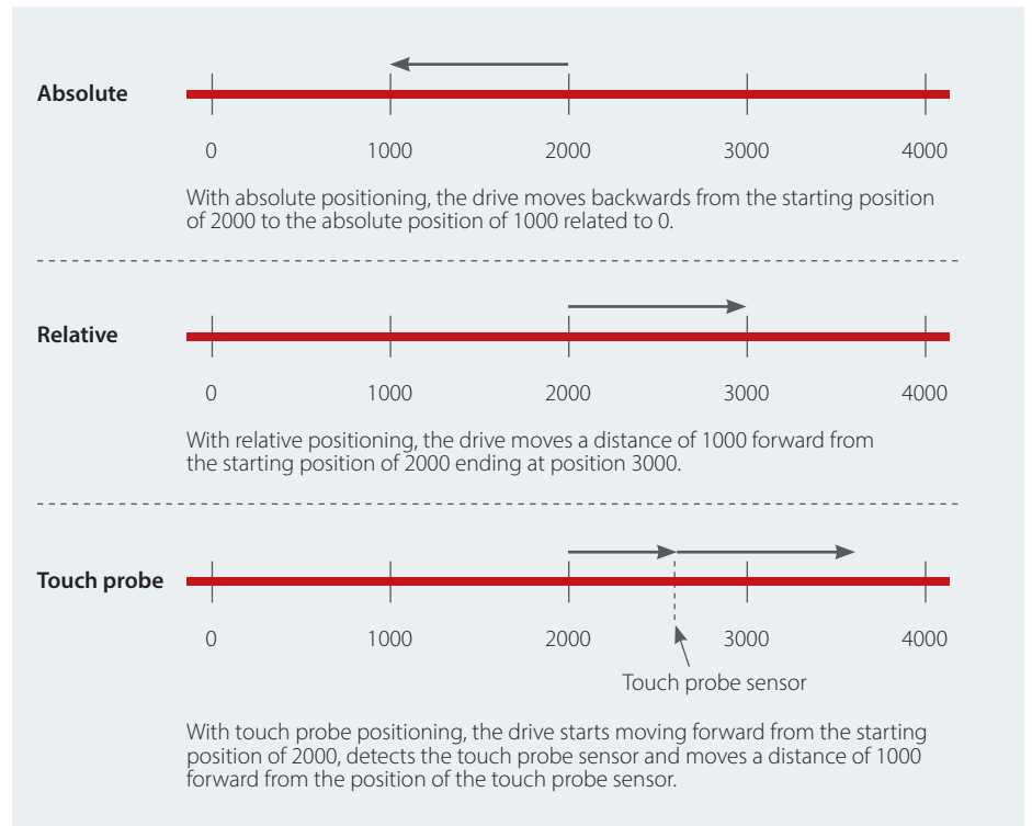
Fig. 3. IMC supports 3 positioning modes
