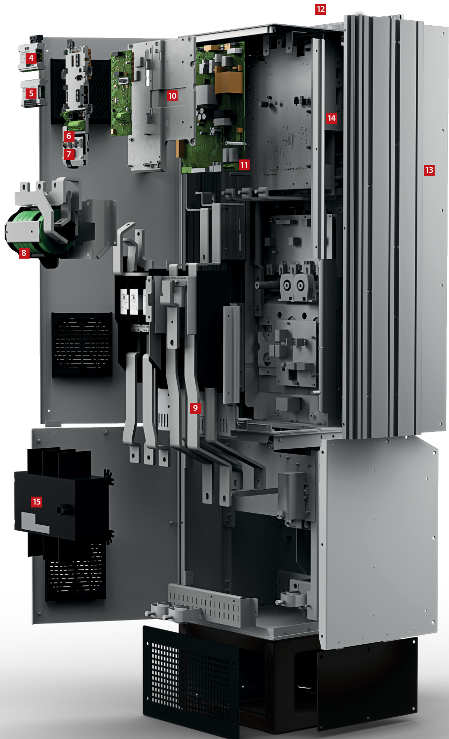
VLT® AutomationDrive FC 302, enclosure size T5
