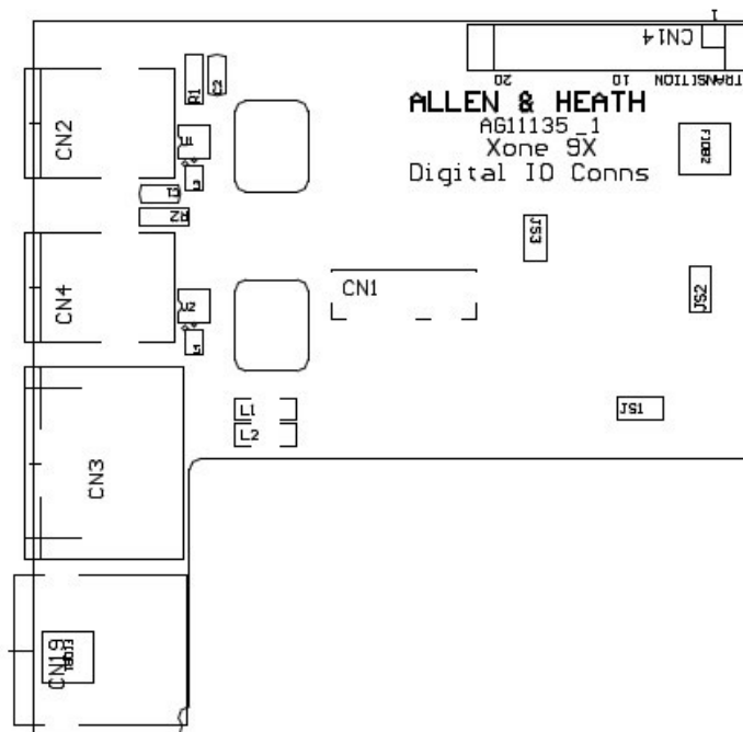
DIGITAL I/O CONN Assembly 004-963 (PCB AG11135)
