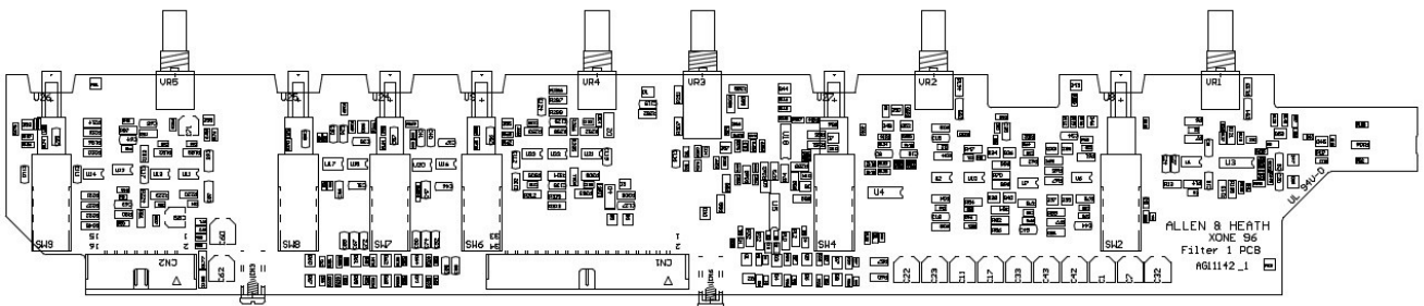
FILTER 1 Assembly 004-697 (PCB AG11142)
