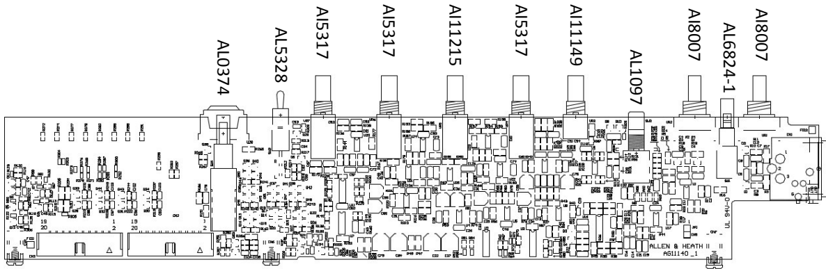
MIC RTN 1 Assembly 004-965 (PCB AG11140)
