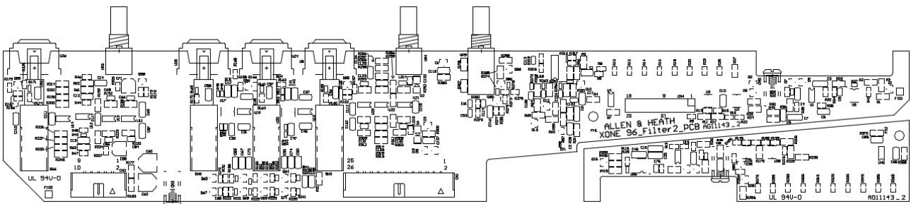
FILTER 2 Assembly 004-968 (PCB AG11143)
