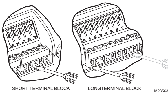
Fig. 10. Removing Terminal Blocks.
