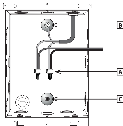
CONNECTION DIAGRAM
