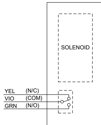
Lock Status Switch Wiring for Fail Safe
