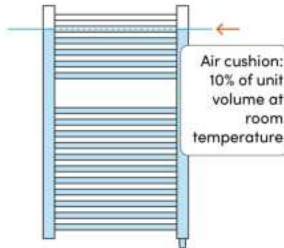
Figure 7 | Air cushion requirement
