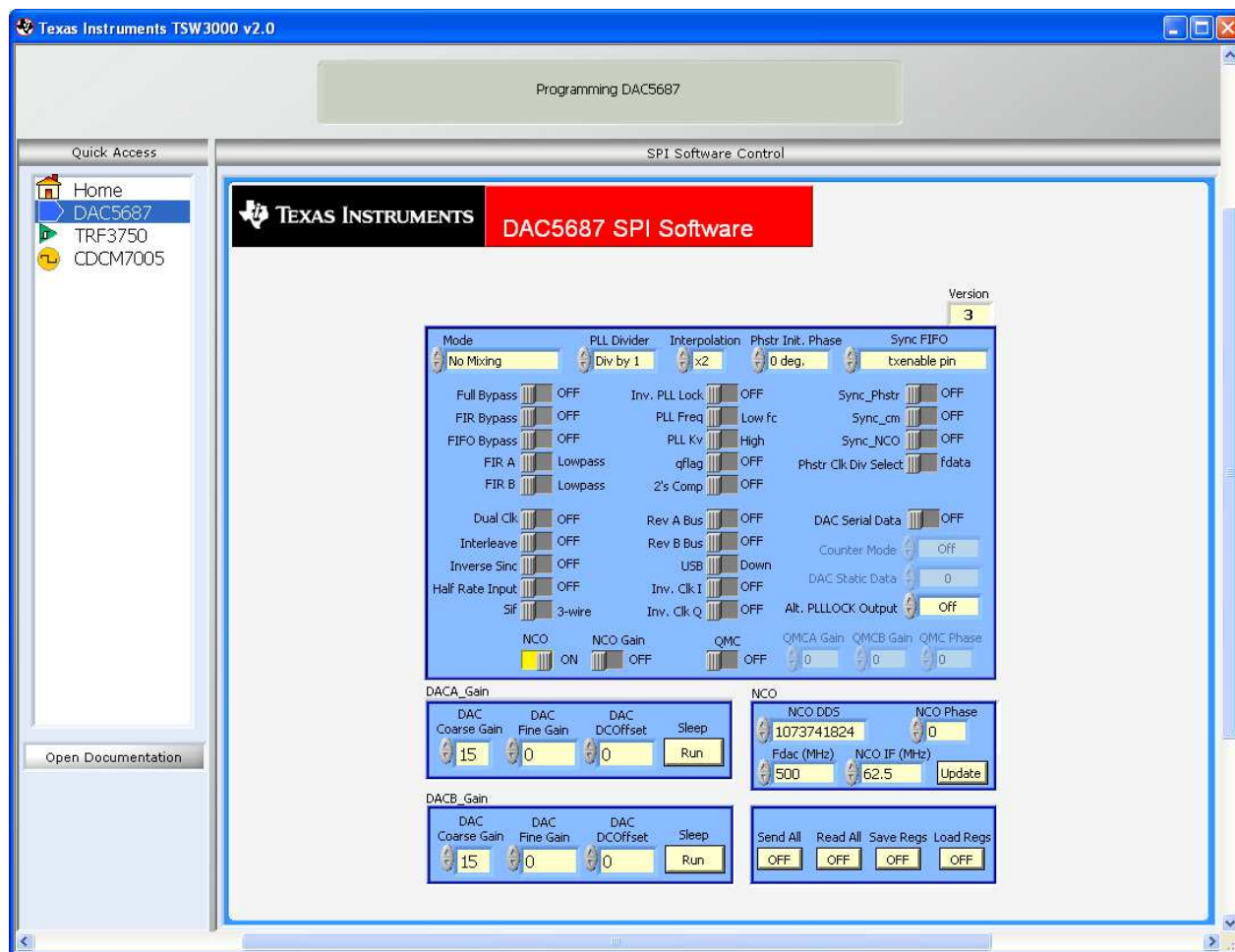
Figure 7. DAC5687 GUI
