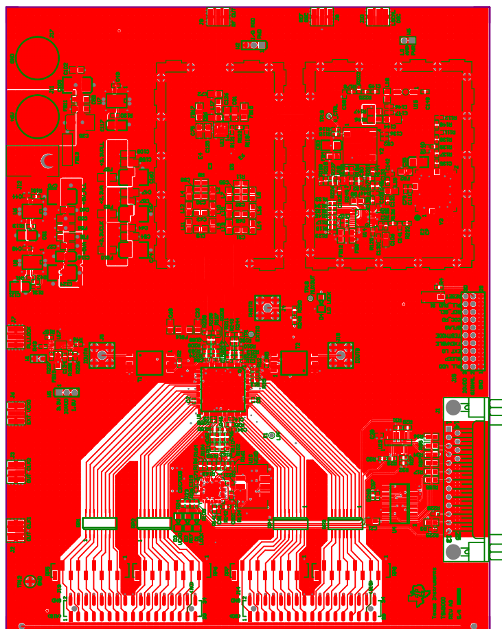
Figure 13. Top Layer
