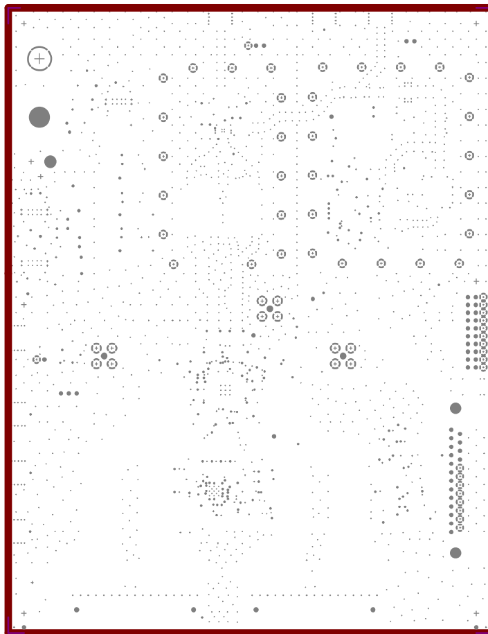
Figure 15. Layer 2
