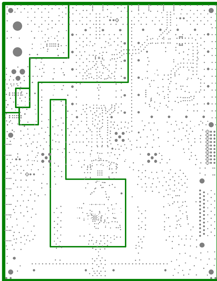
Figure 16. Layer 3
