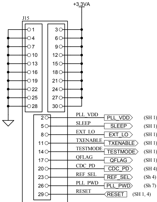
3 ROW 30 PIN CONNECTOR
