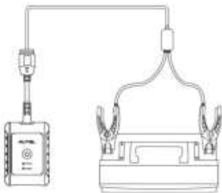
Figure 11-4 Battery Tester Connection Example 2
