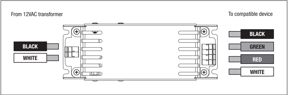
Figure 5. RGB Wiring
