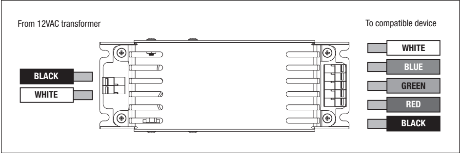
Figure 6. RGBW Wiring
