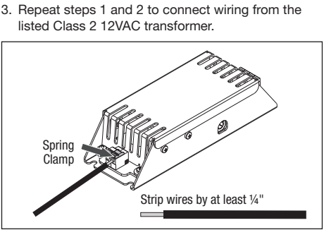
Figure 4. Wire Stripping and Insertion
